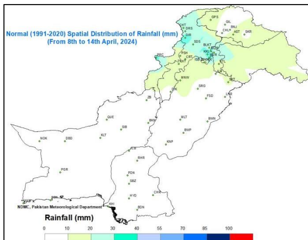
Figure 9: Spatial Distribution of Normal Rainfall (mm)
