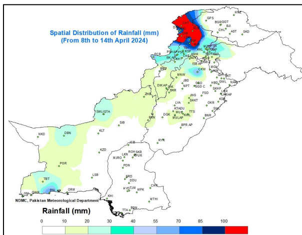
Figure 5: Spatial Distribution of rainfall(mm)
