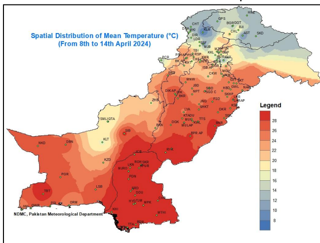
Figure 7: Spatial Distribution of Mean Temperature(°C)
