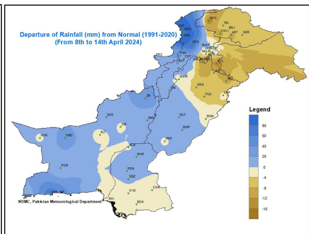
Figure 6: Departure of rainfall(mm)
