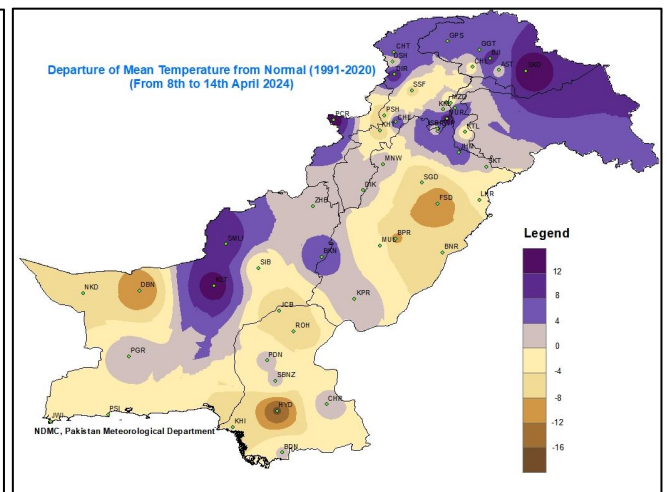
Figure 8: Departure of Mean Temperature(°C)
