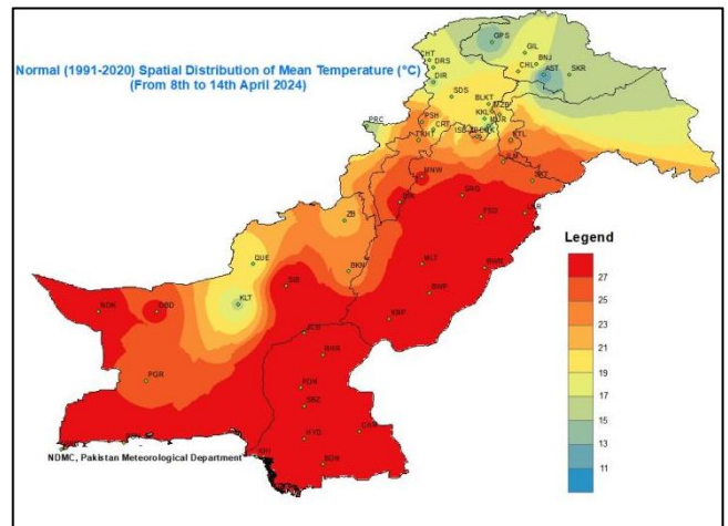
Figure 10: Spatial Distribution of Normal Mean Temperature (°C)
