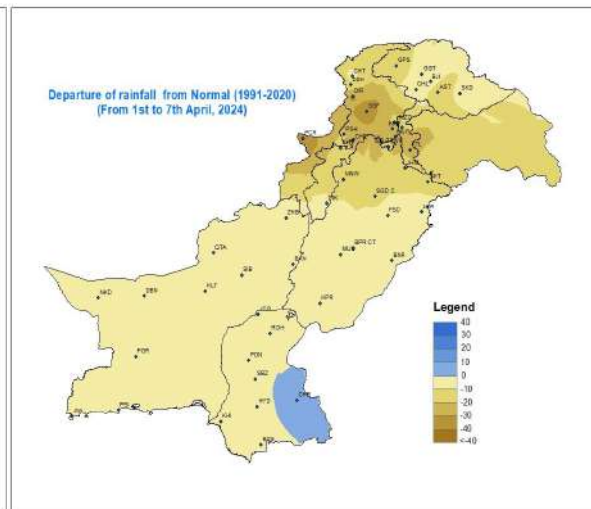
Figure 6: Departure of rainfall(mm)
