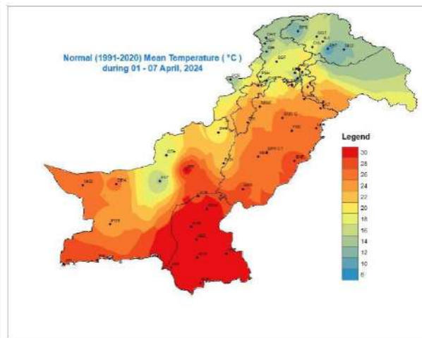
Figure 10: Spatial Distribution of Normal Mean Temperature(°C)
