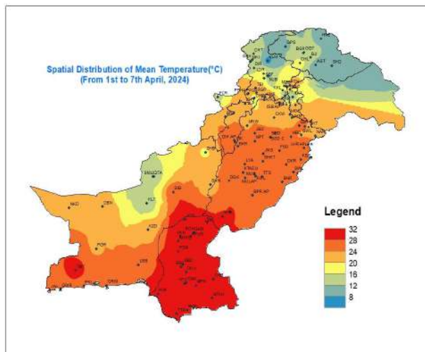
Figure 7: Spatial Distribution of Mean Temperature(°C)
