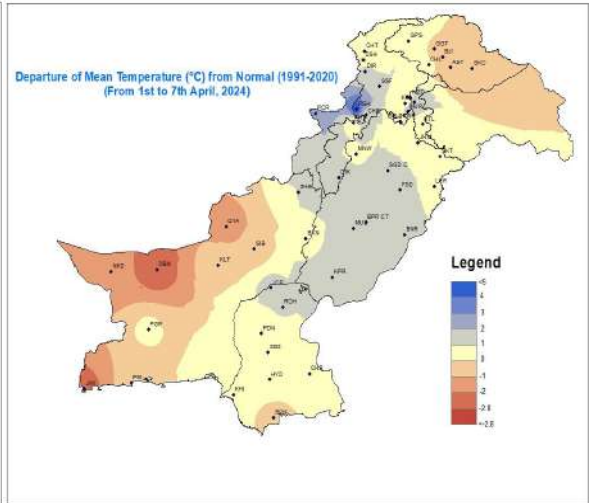
Figure 4: Departure of Mean Temperature(°C)
