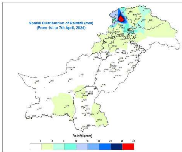
Figure 5: Spatial Distribution of rainfall(mm)
