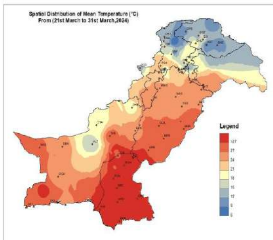
Figure 7: Spatial Distribution of Mean Temperature(°C)
