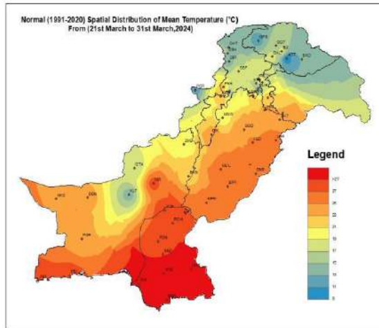
Figure 10: Spatial Distribution of Normal Mean Temperature(°C)
