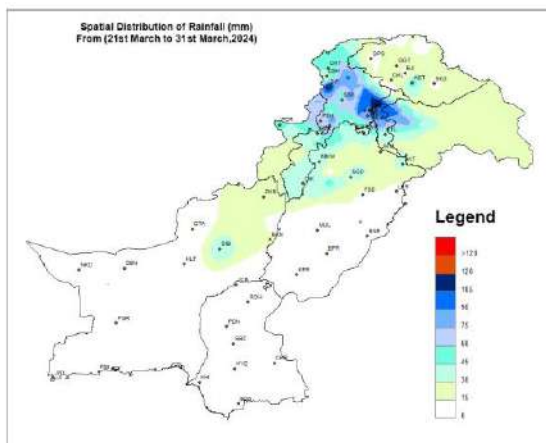
Figure 5: Spatial Distribution of rainfall(mm)
