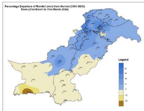
Figure 6: Departure of rainfall(%)
