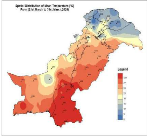
Figure 3: Spatial Distribution of Mean Temperature(°C)
