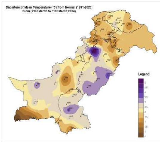
Figure 4: Departure of Mean Temperature(°C)
