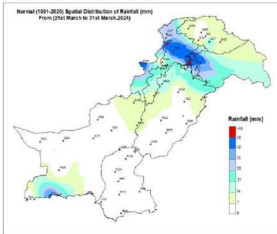
Figure 9: Spatial Distribution of Normal Rainfall(mm)
