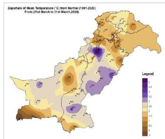
Figure 8: Departure of Mean Temperature(°C)
