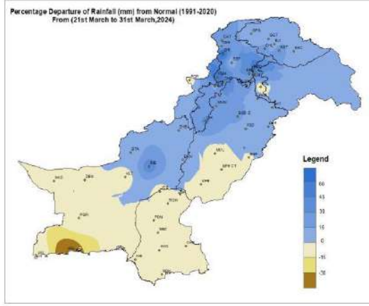
Figure 2: Departure of rainfall (%)
