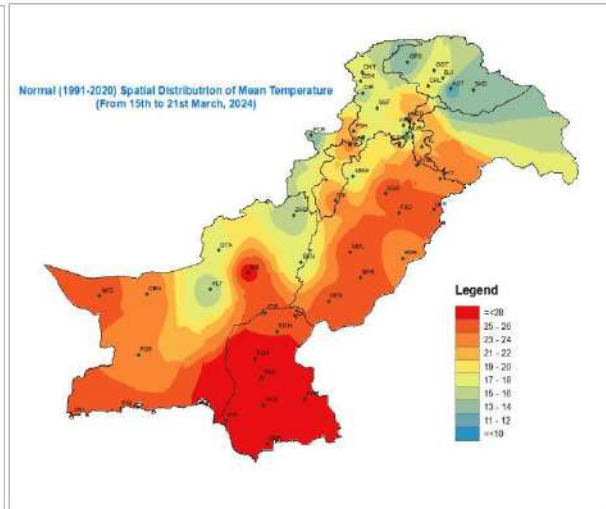
Figure 10: Spatial Distribution of Normal Mean Temperature (°C)
