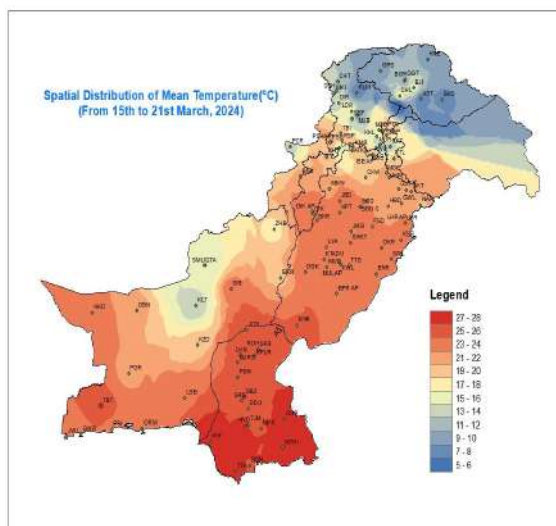
Figure 7: Spatial Distribution of Mean Temperature(°C)
