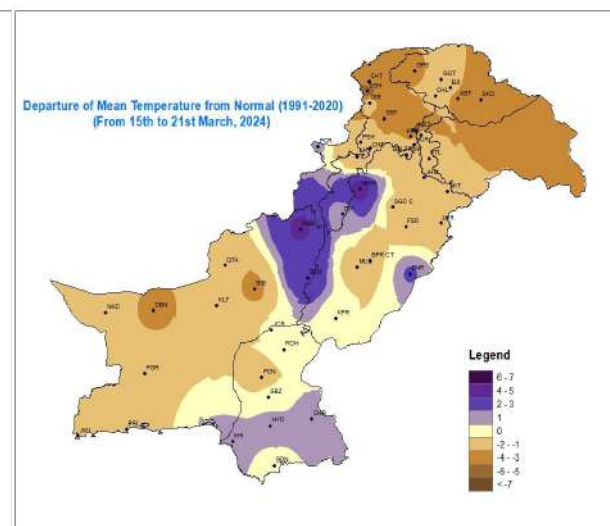
Figure 8: Departure of Mean Temperature(°C)
