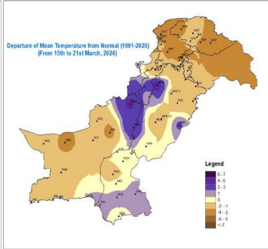
Figure 4: Departure of Mean Temperature(°C)
