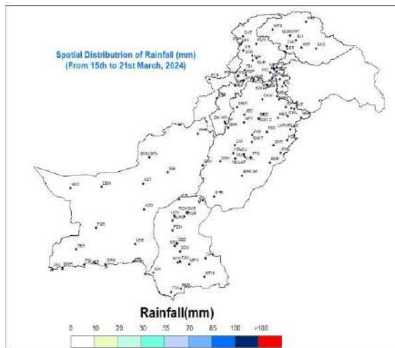
Figure 5: Spatial Distribution of rainfall(mm)
