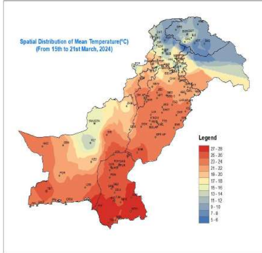
Figure 3: Spatial Distribution of Mean Temperature(°C)
