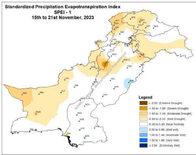
Figure 1 Standardized Precipitation Evapotranspiration Index (SPEI-1)
